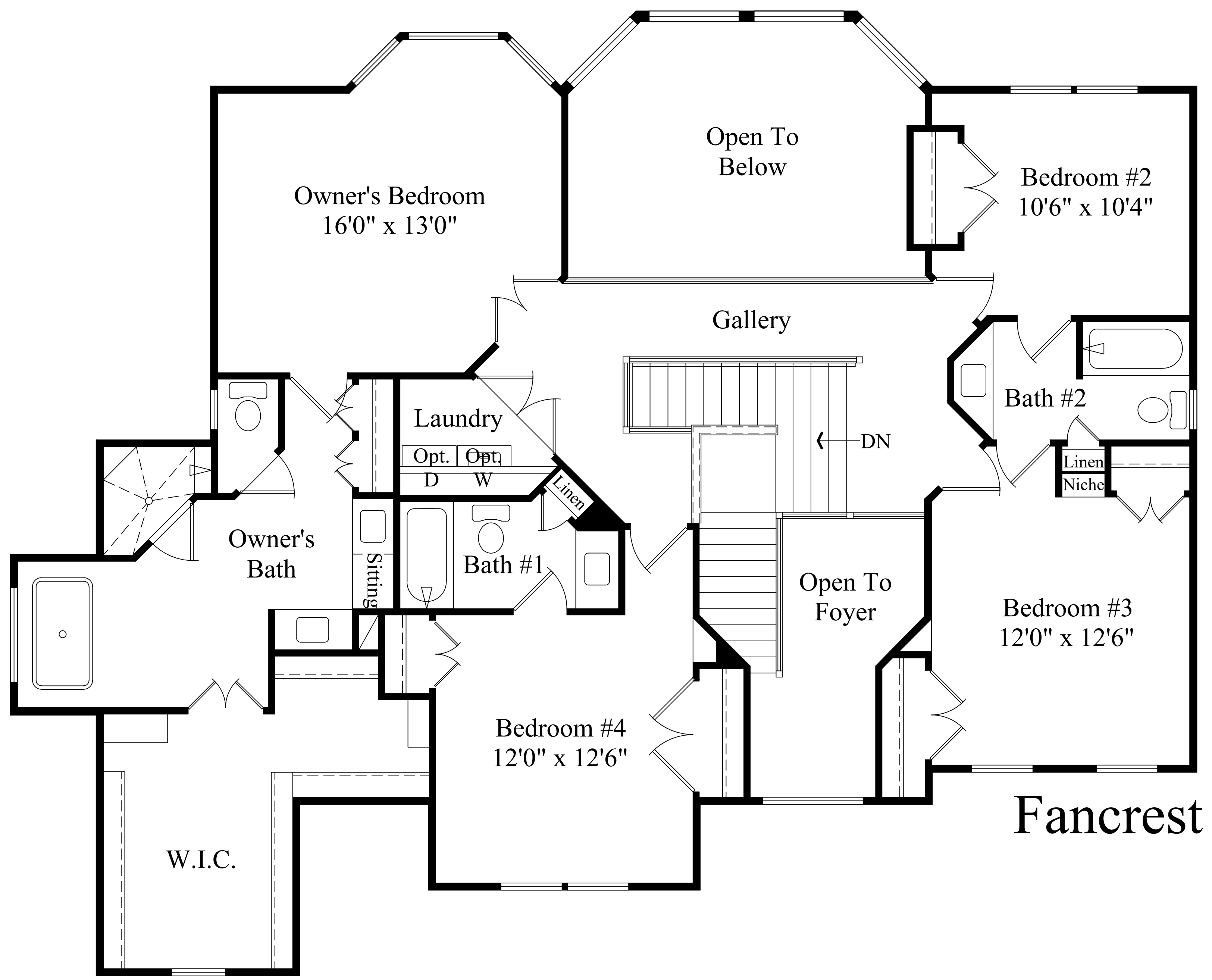
2nd Floor
