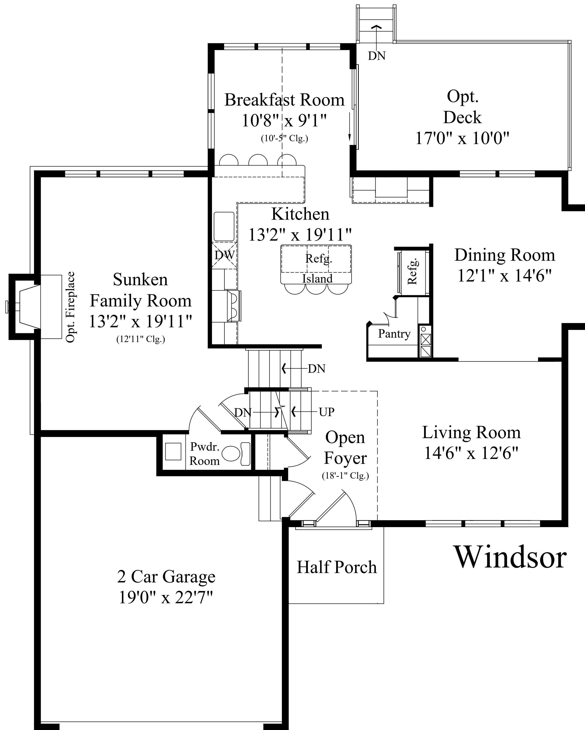
1st Floor
