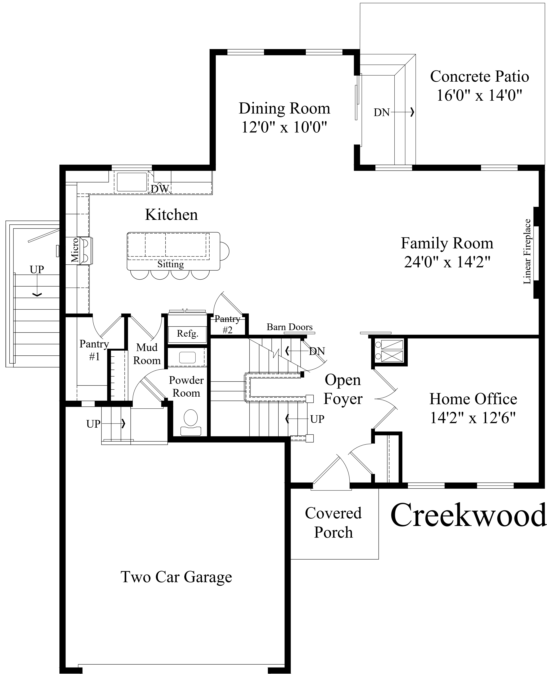
1st Floor
